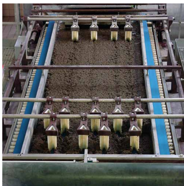
Belt filter in a sewage facility for sludge dewatering
