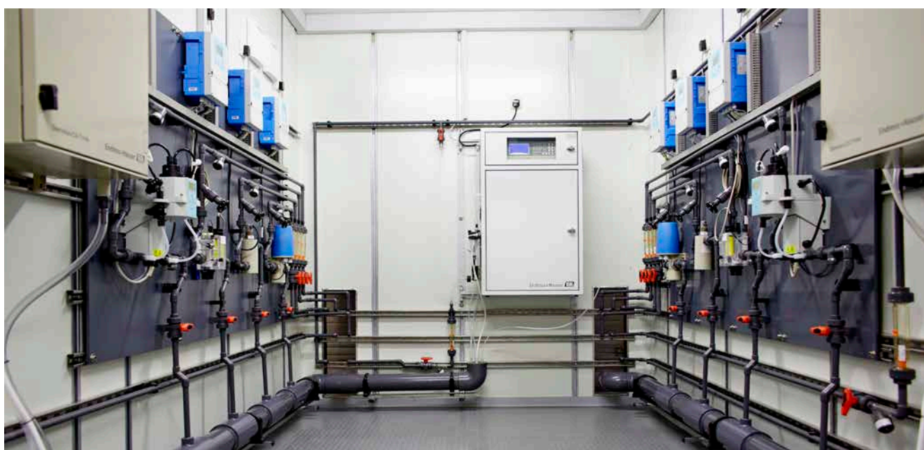
Container solution of Endress+Hauser for efficient water management in production and auxiliary circuits
